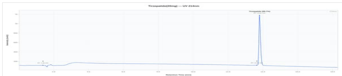
Tirzepatide GLP2 20mg - GLP2-2026-06-20mg-02: UV Chromatogram
